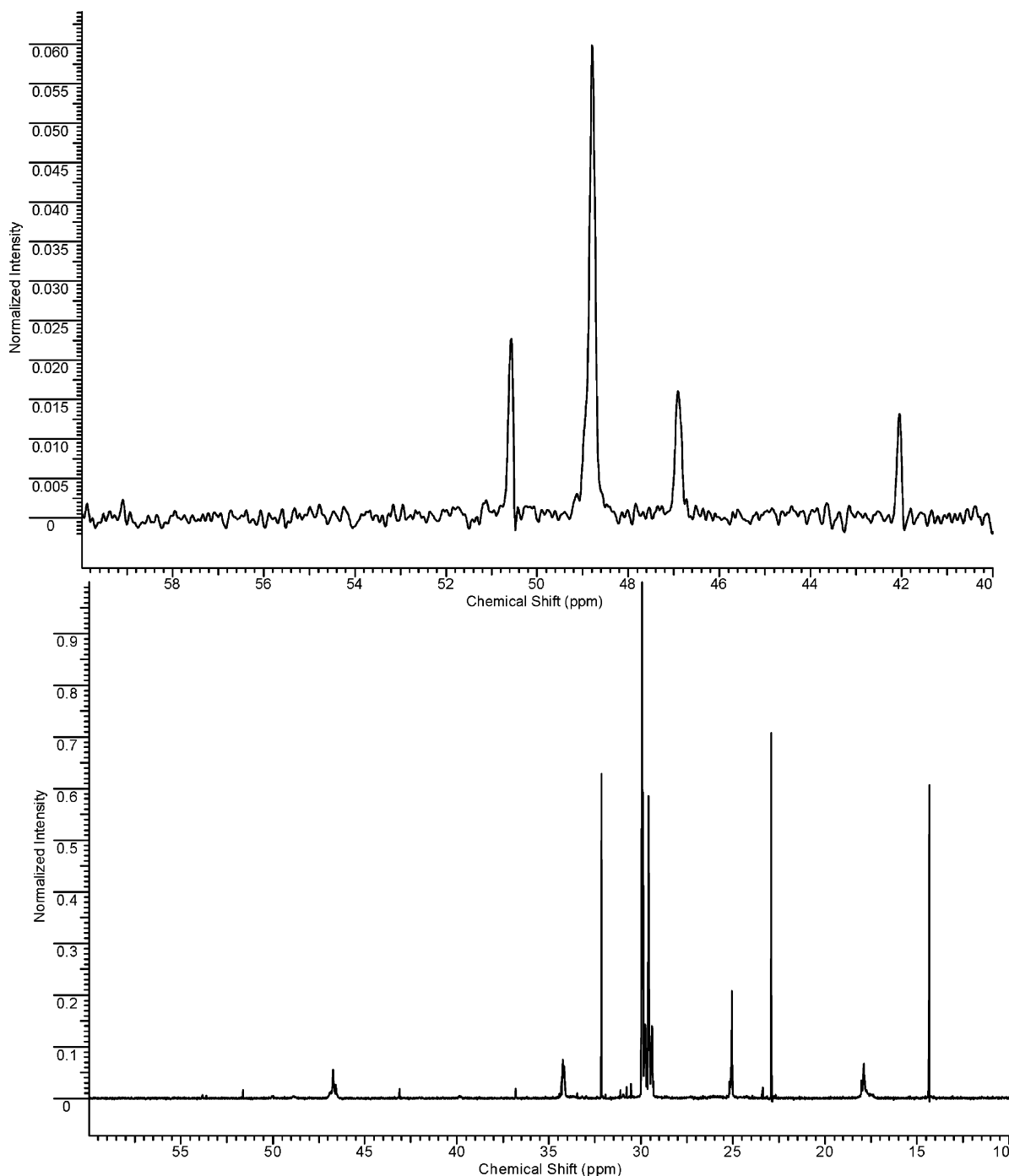
Figure 1. 13 C NMR spectra for the fractionated core BH40-pr in d 6 -DMSO (top) and compound 3 in CDCl 3 (bottom).
